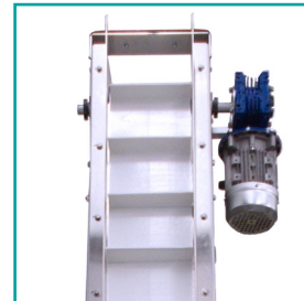
Close up of the new motor mount on the 2015 EP-08
